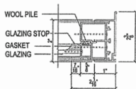
A CITIQUIET REMOVABLE PICTURE WINDOW - JAMB DETAIL SCALE 1/4" = 1"
