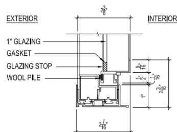
D CITIQUIET HINGED WINDOW SILL DETAIL SCALE: 1"=1"
