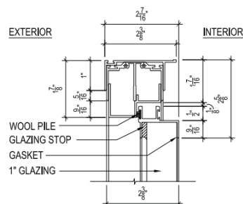
C CITIQUIET HINGED WINDOW HEADER DETAIL SCALE: 1"=1"
