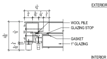
A CITIQUIET HINGED WINDOW JAMB DETAIL SCALE: 1"=1"
