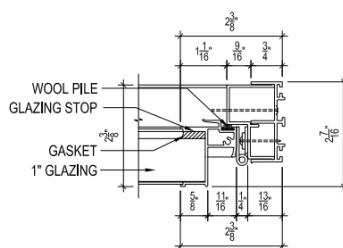
B CITIQUIET HINGED WINDOW JAMB DETAIL SCALE: 1"=1"
