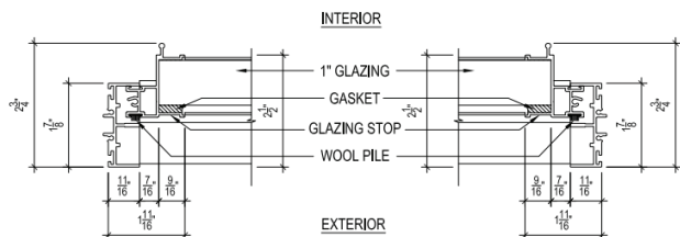
A CITIQUIET REMOVABLE PICTURE WINDOW - JAMB DETAIL LEFT SCALE: 1\"/>
