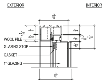
B CITIQUIET REMOVABLE PICTURE WINDOW - HEADER DETAIL SCALE: 1\"/>
