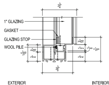
C CITIQUIET REMOVABLE PICTURE WINDOW - SILL DETAIL SCALE: 1\"/>
